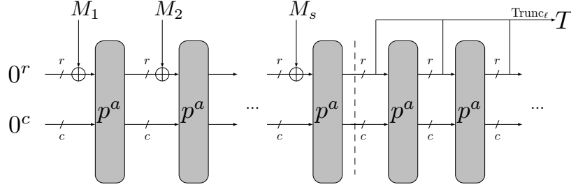
Figure 1: Sponge function
