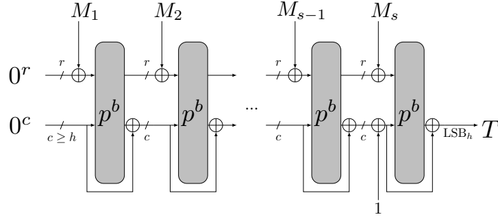
Figure 2: Feed-forward Sponge function
